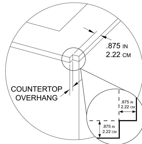
COUNTER TOP NOTCH DETAIL
